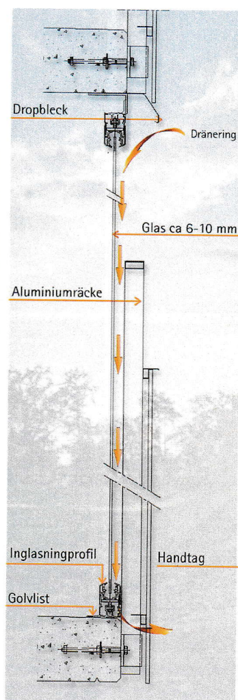
Principritning system D
